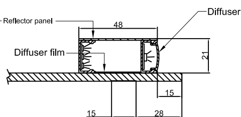
LED holder+soft silicone diffuser Section A-A
