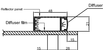
LED holder+soft silicone diffuser
