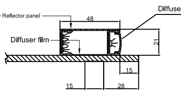
LED holder+soft silicone diffuser Section A-A
