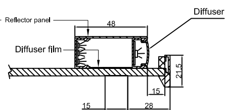
LED holder+soft silicone diffuser Section A-A
